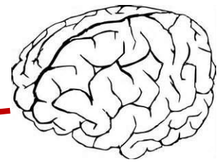
Hydrated Brain
